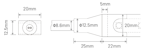
IP68 Silicone Injection-moulded Front Connector-End
